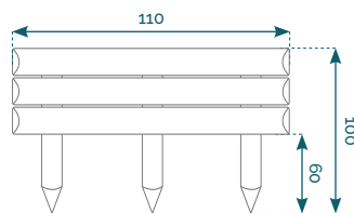
BOPLDR-100x60-110
